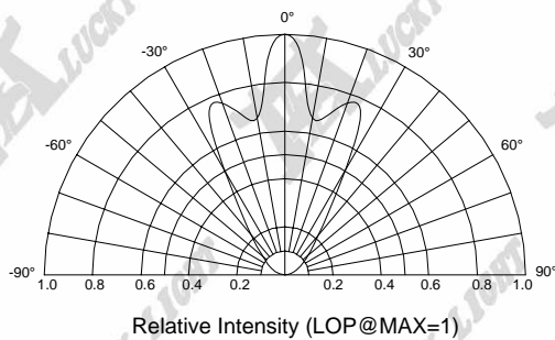
Beam Pattern
